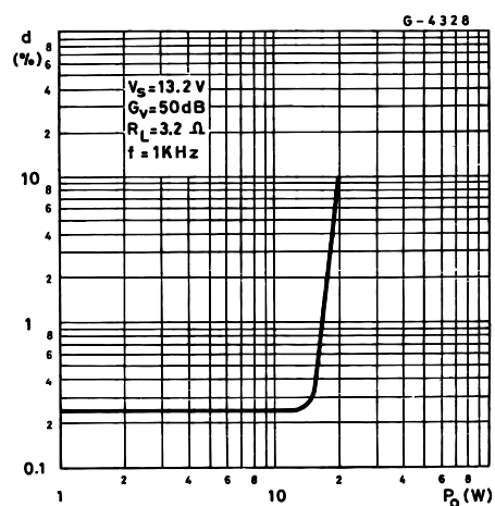
Figure 5 : Distortion versus Output Power (bridge amplifier)
